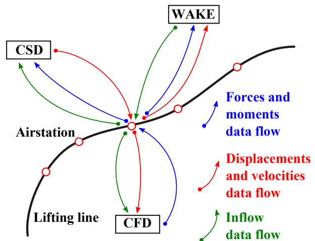
Figure 4: Schematics of the aerodynamics interface.
